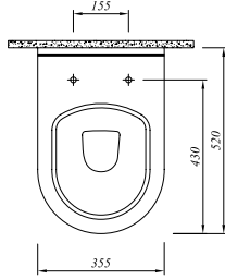
71125334xx İdea Universal Asma Klozet [Taharet Delikli] İdea Universal Wall Hung WC Pan [With Cleaning Pipe] 71125363xx İdea Universal Asma Klozet [Taharet Deliksiz] İdea Universal Wall Hung WC Pan [Without Cleaning Pipe] 70113720xx Klozet Kapağı Seat & Cover 70113728xx Yavaş Kapanan Klozet Kapağı Soft Close Seat & Cover
