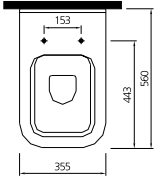
71110334xx Babel Universal Asma Klozet [Taharet Delikli] Babel Universal Wall Hung WC Pan [With Cleaning Pipe] 71110363xx Babel Universal Asma Klozet [Taharet Deliksiz] Babel Universal Wall Hung WC Pan [Without Cleaning Pipe] 70110720xx Babel Klozet Kapağı Babel Seat & Cover 70110728xx Babel Yavaş Kapanan Klozet Kapağı Babel Soft Close Seat & Cover
